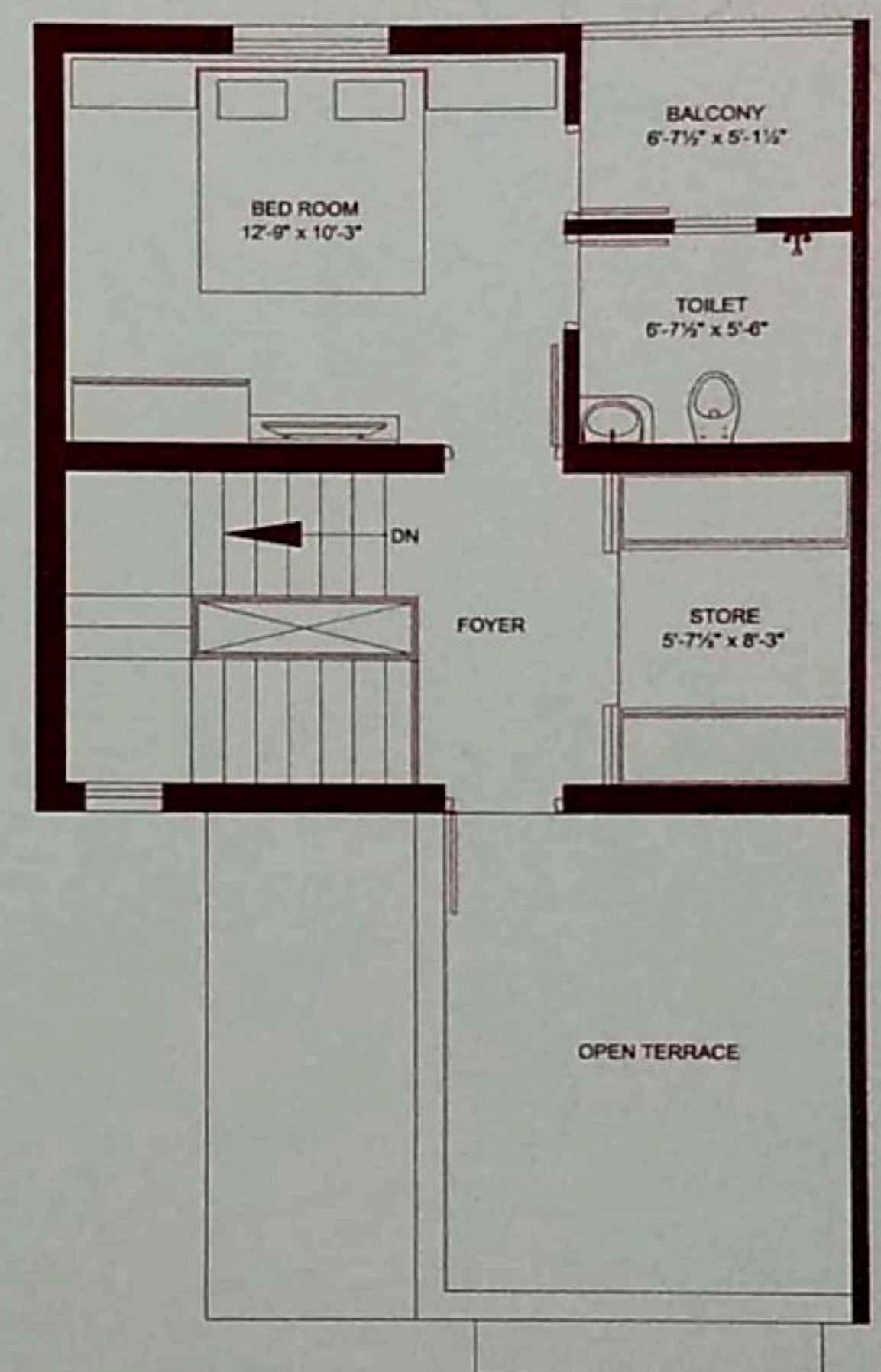
SECOND FLOOR
