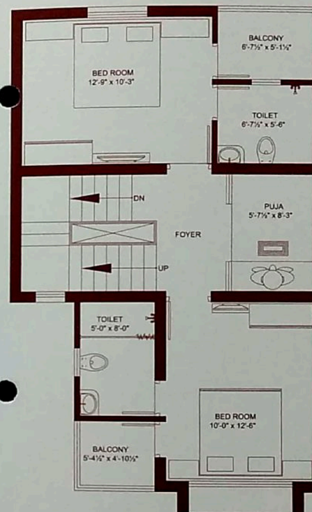
FIRST FLOOR
